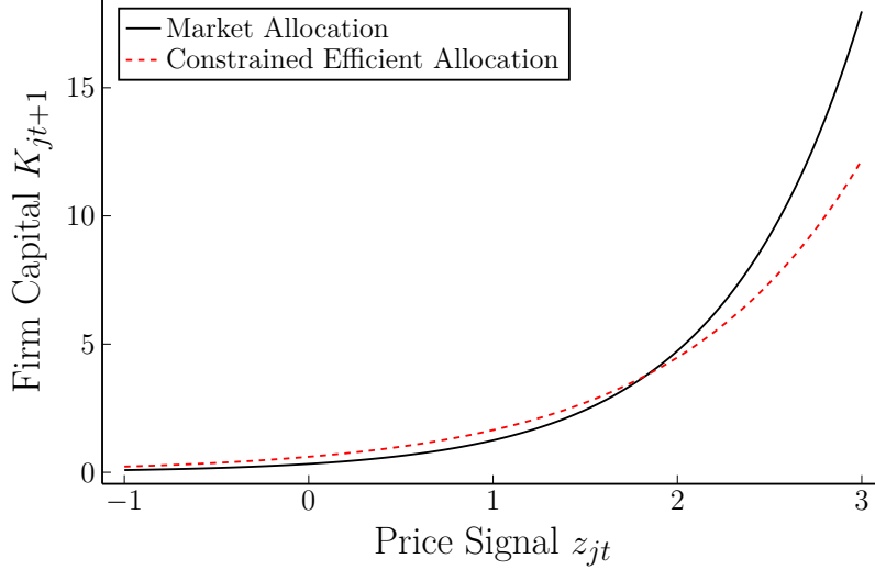
Figure 5: Market allocation of capital K_{jt} as in (25) and the constrained efficient allocation K_{jt}^{eff} as in (28).
