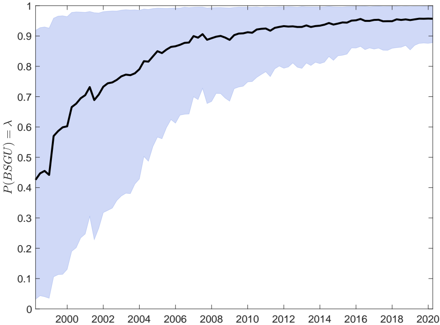
Figure 3: Model Weights: Expectations Traps vs Secular Stagnation
