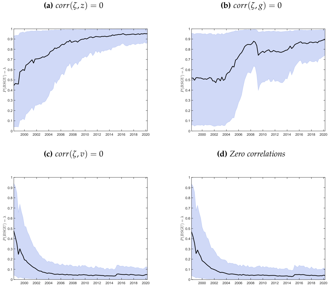
Figure 5: Model Weights: Role of Sunspots
