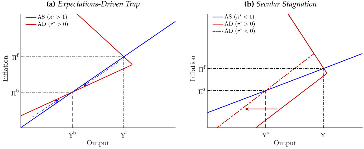
Figure 1: Steady State Representation
