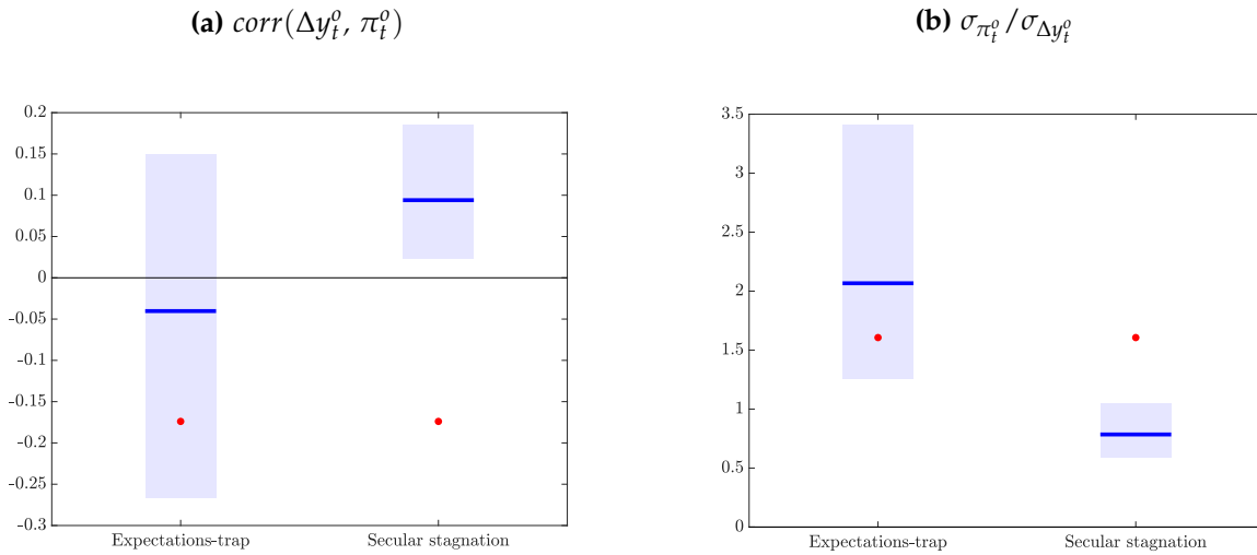
Figure 6: Moments: models vs data
